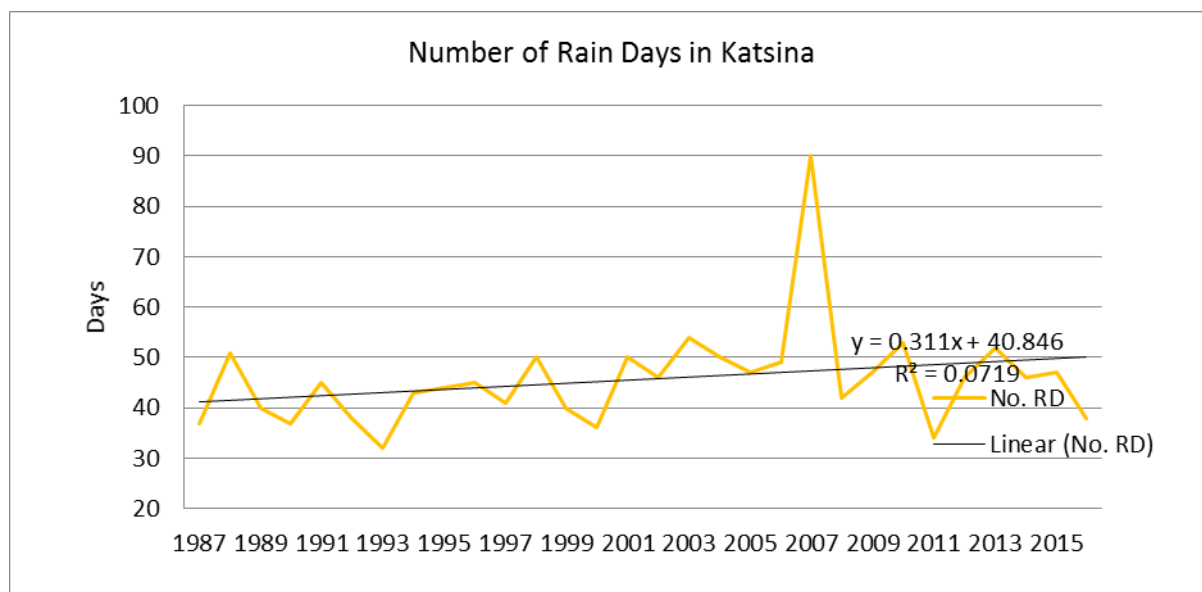
Figure 4. Trend of Number of Actual Rain Days in Katsina
