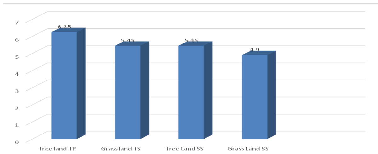
Figure 6: pH Recorded in the Study Area Source: Field Work, 2022.
