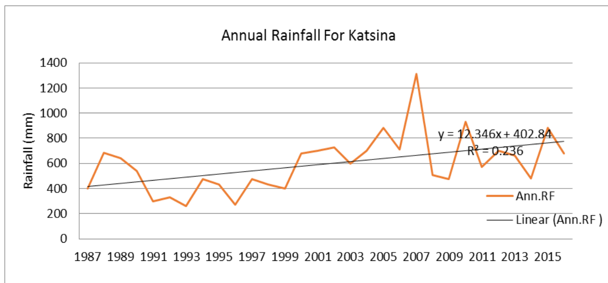
Figure 2. Trend of Total Annual Rainfall in Katsina.
