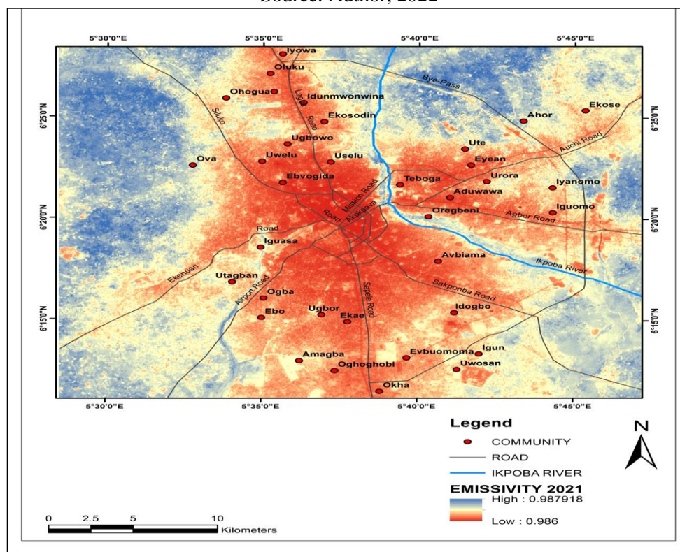
Figure 9: Land Surface Emissivity of Benin City, 2021
