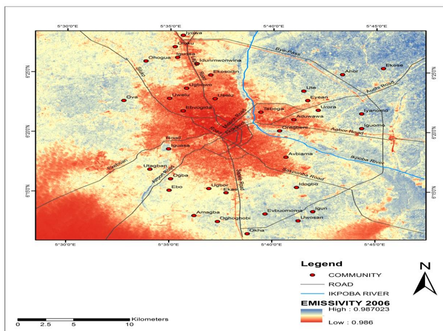
Figure 8: Land Surface Emissivity of Benin City, 2006
