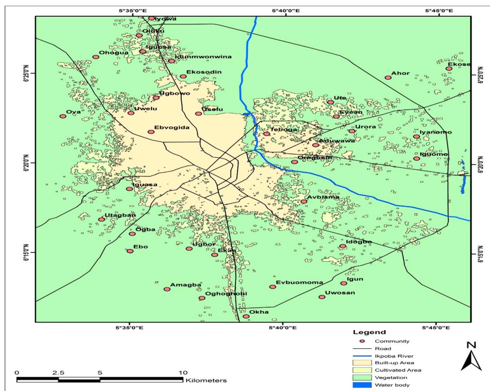
Figure 3: Land Use/Land Cover Profile of Benin City in 1991 Source: Author, 2022.
