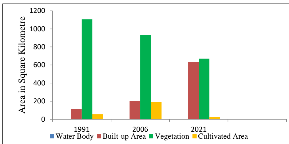
Figure 6: Spatio-Temporal changes in Land use/Land cover of Benin City (1991-2021)
