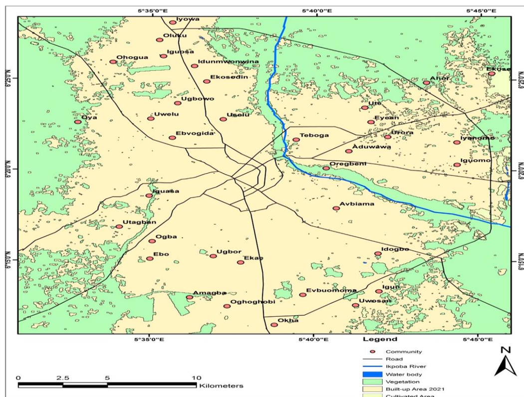
Figure 5: Land Use/Land Cover Profile of Benin City in 2021
